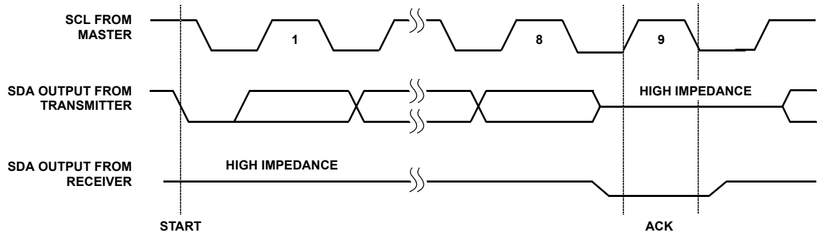
FIGURE 20. ACKNOWLEDGE RESPONSE FROM RECEIVER
