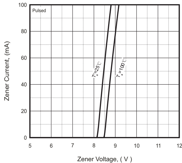
Fig.3 - Reverse Characteristics
