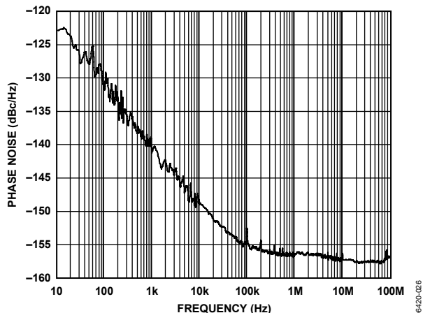
Figure 31. Phase Noise (Additive) LVPECL @ 245.76 MHz, Divide-by-1
