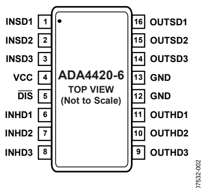
Figure 3. 16-Lead QSOFP Pin Configuration
