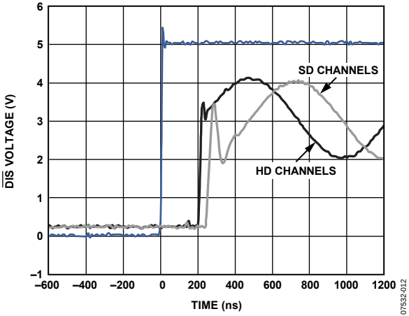
Figure 13. Enable Time
