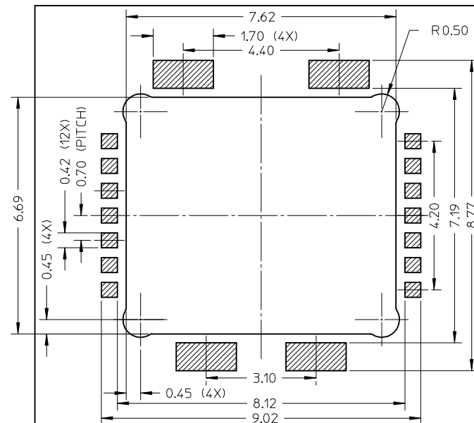
B TYPE PCB LAYOUT FOR PRODUCT NO. 1052000006,1052000007, 1052000008,1052000009 TOLERANCE:0.05mm
