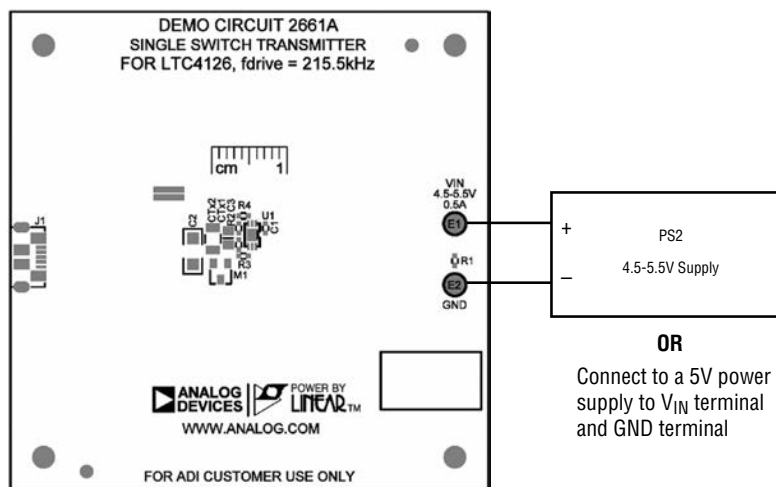
Figure 6. DC2661A Top
