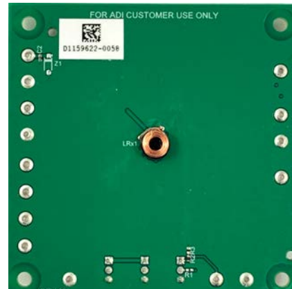
Figure 9. DC2662A Top/Bottom
