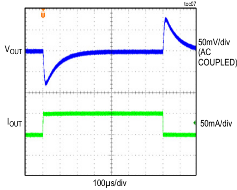
LOAD CURRENT TRANSIENT RESPONSE ( V_{IN} = 24V , V_{OUT} = 5V , I_{OUT} = 0.05A TO 0.1A )
