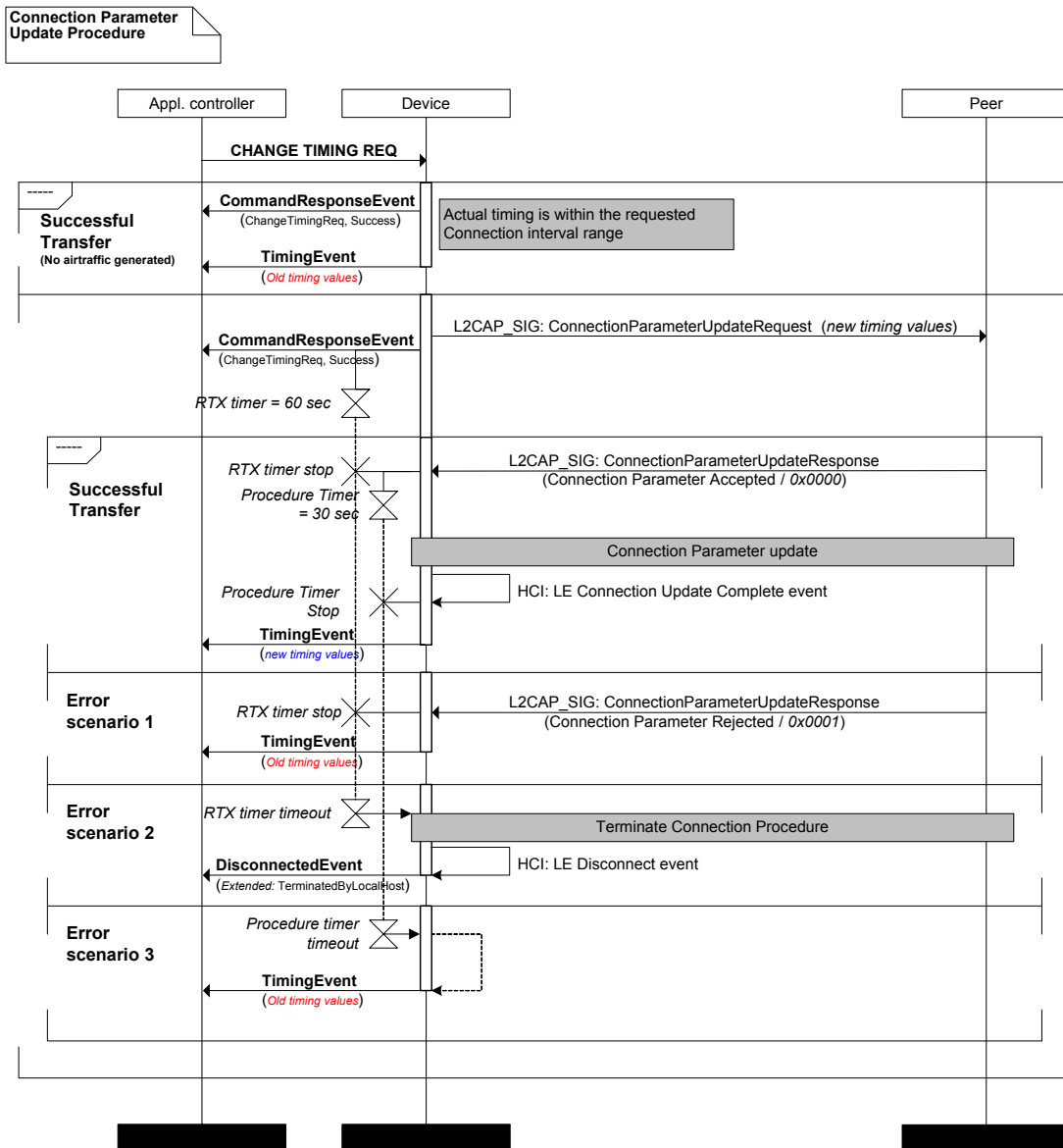
Figure 51. ChangeTimingRequest MSC
