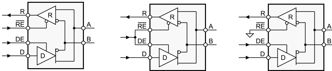
Figure 17. Half-Duplex Transceiver Configurations
