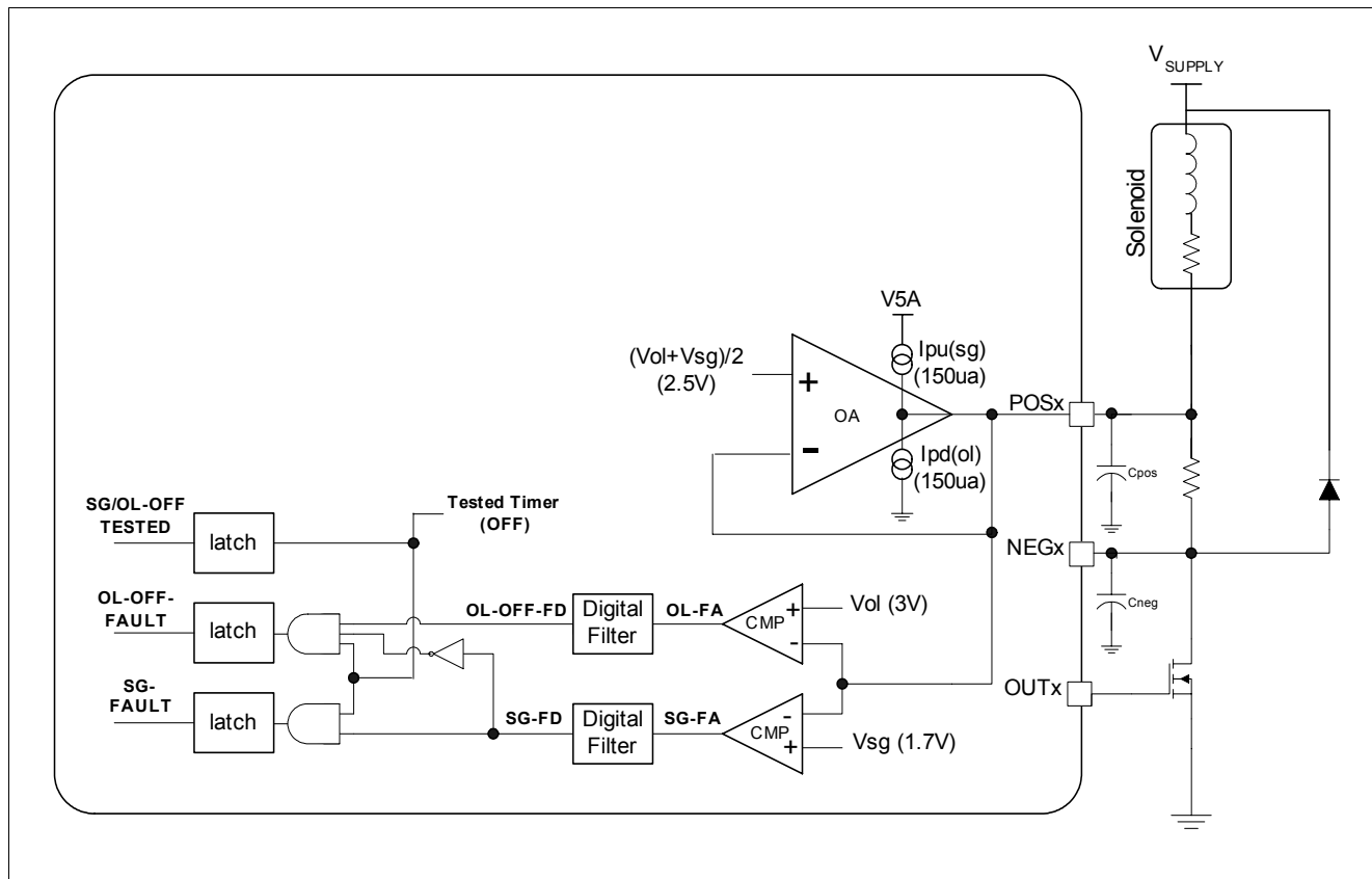
Figure 12 Off-State Diagnostics
