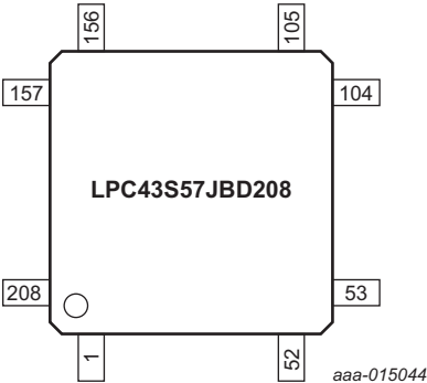
Fig 4. Pin configuration LQFP208 package
