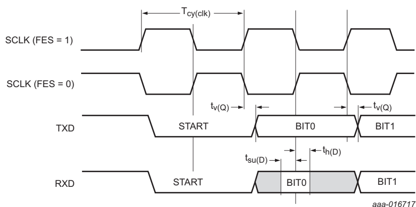
Fig 30. USART timing
