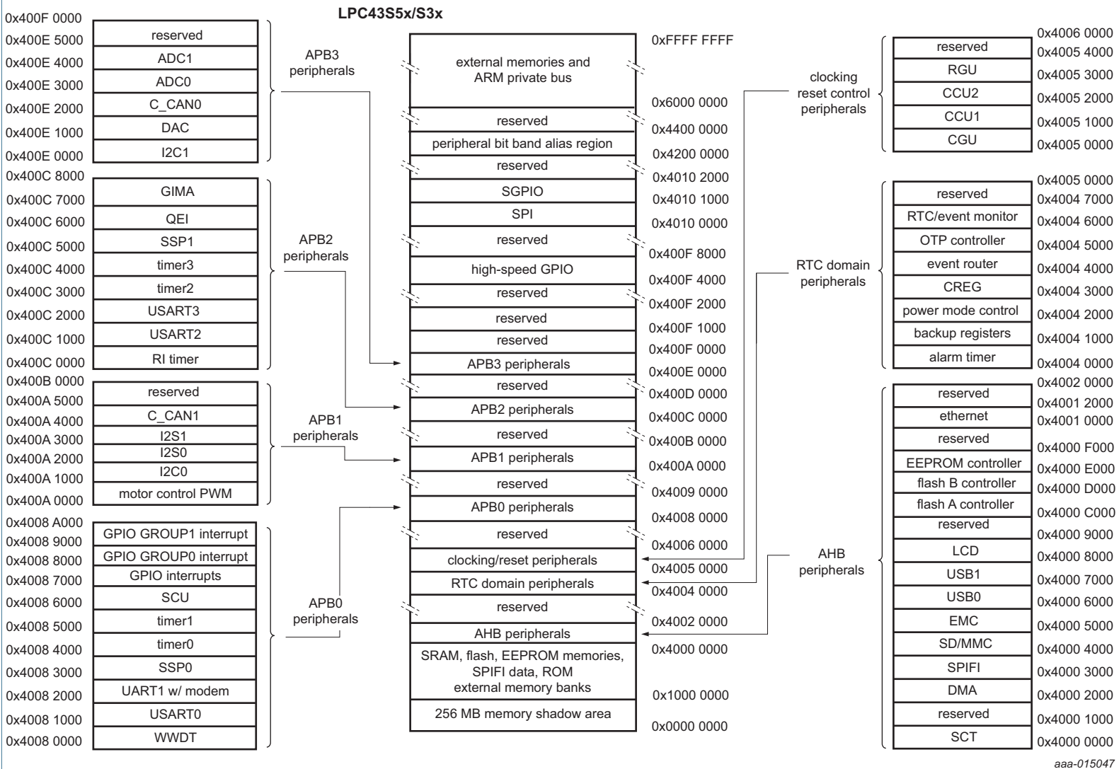
Fig 8. LPC4335x/S3x Memory mapping (peripherals)
