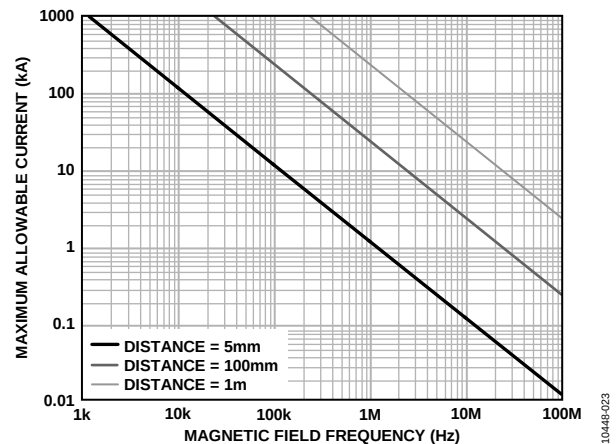
Figure 23. Maximum Allowable Current for Various Current-to- ADuM7640/ADuM7641/ADuM7642/ADuM7643 Spacings
