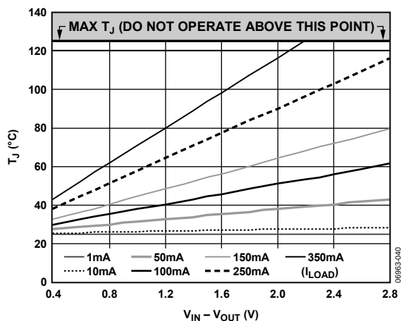
Figure 40. 500 mm 2 of PCB Copper, T_A = 25^{\circ}\text{C} , TSOT
