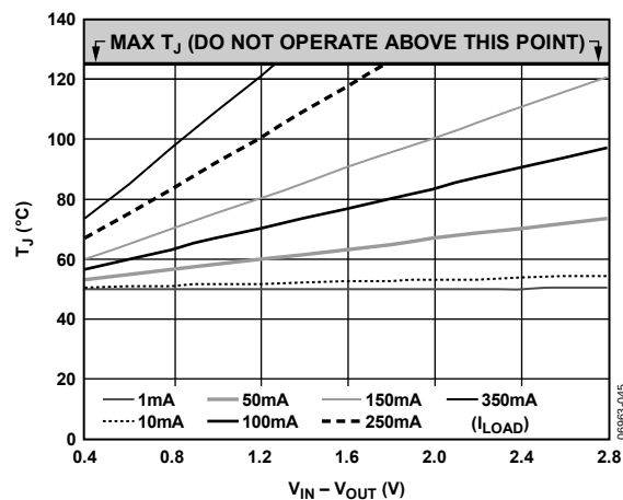
Figure 45. 0 mm 2 of PCB Copper, T_A = 50^{\circ}\text{C} , TSOT
