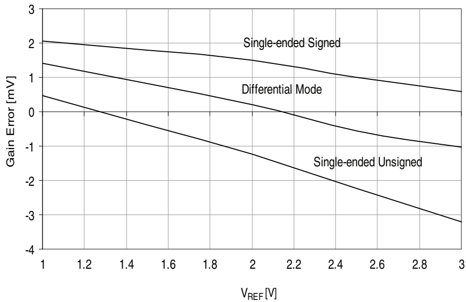
Figure 37-294. Gain error vs. V_{REF} T = 25^{\circ}\text{C} , V_{CC} = 3.6\text{V} , ADC sampling speed = 500kps
