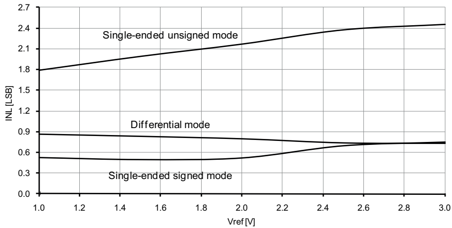
Figure 37-204. INL error vs. external V_{REF} . T = 25^\circ\text{C} , V_{CC} = 3.6V , external reference.
