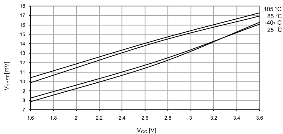
Figure 37-137. Analog comparator hysteresis vs. V_{CC} .
