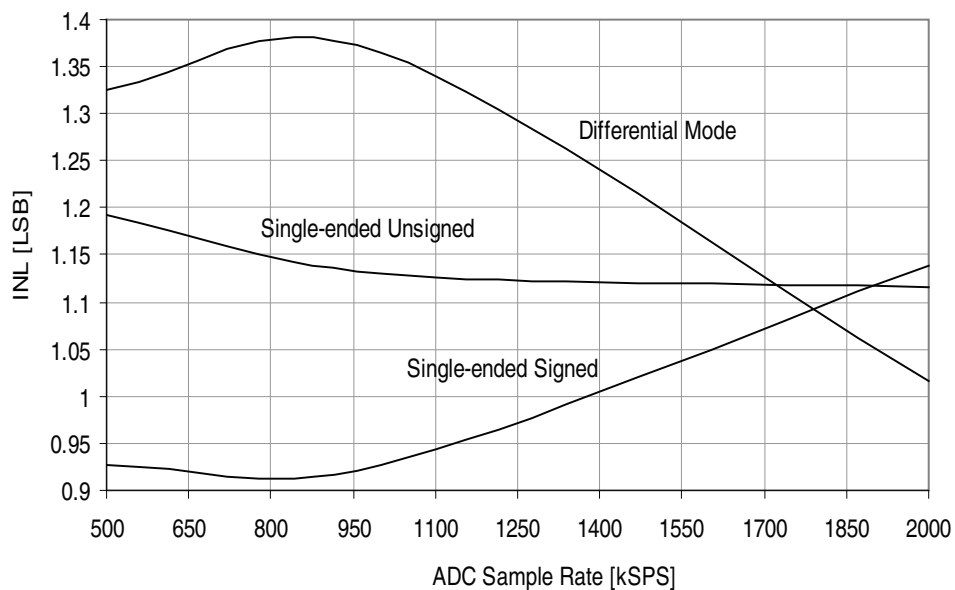
Figure 37-37. INL error vs. sample rate. T = 25^{\circ}\text{C} , V_{CC} = 3.6\text{V} , V_{REF} = 3.0\text{V} external.
