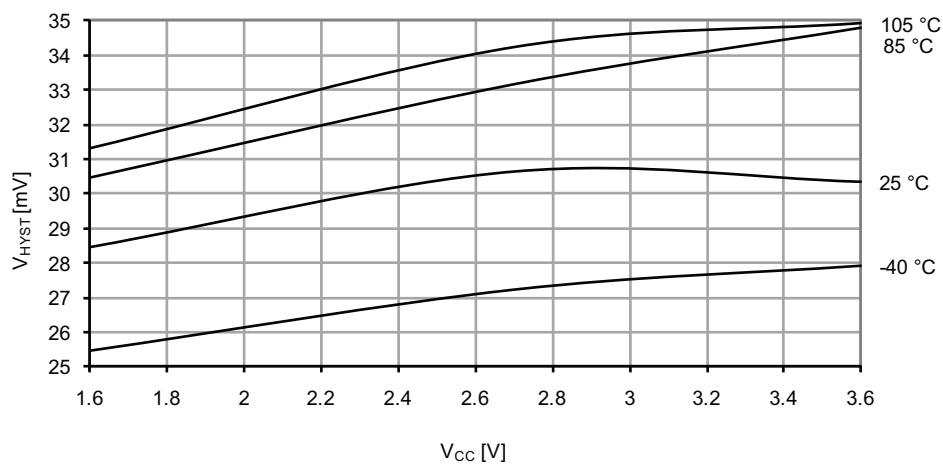
Figure 37-53. Analog comparator hysteresis vs. V_{CC} .
