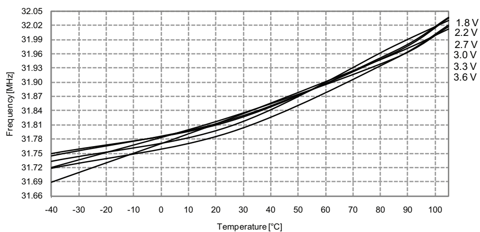
Figure 37-329. 32MHz internal oscillator frequency vs. temperature DPLL enabled, from the 32.768kHz internal oscillator
