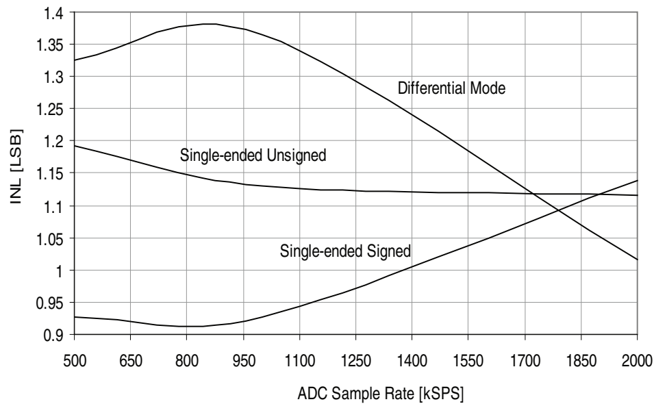
Figure 37-121. INL error vs. sample rate. T = 25^{\circ}\text{C} , V_{CC} = 3.6\text{V} , V_{REF} = 3.0\text{V} external.
