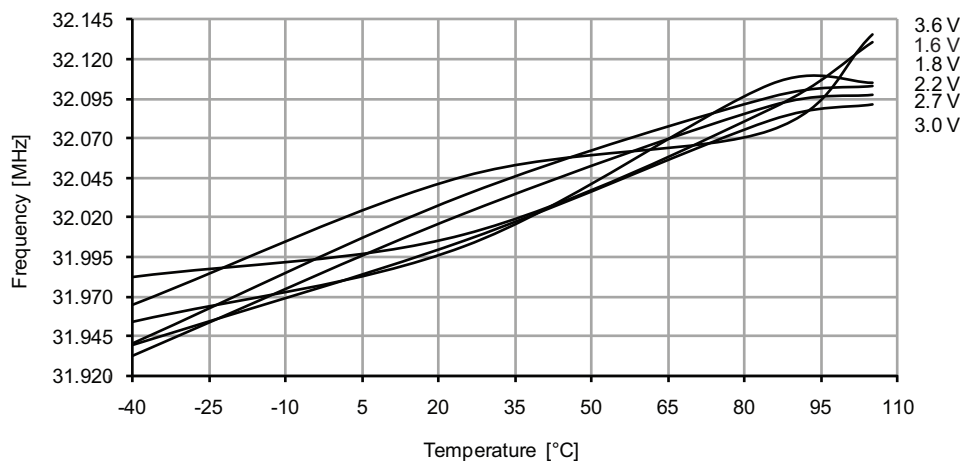
Figure 37-77. 32MHz internal oscillator frequency vs. temperature. DFLL enabled, from the 32.768kHz internal oscillator.
