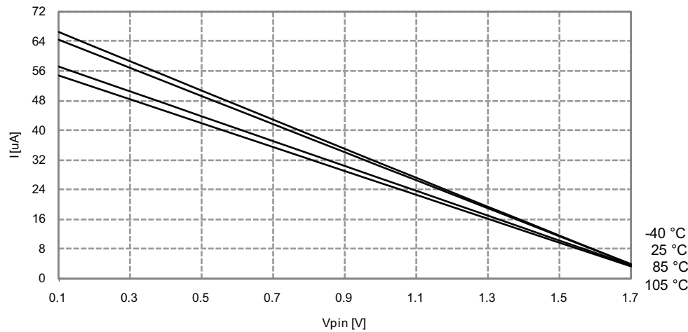
Figure 37-273. I/O pin pull-up resistor current vs. input voltage. V_{CC} = 1.8V
