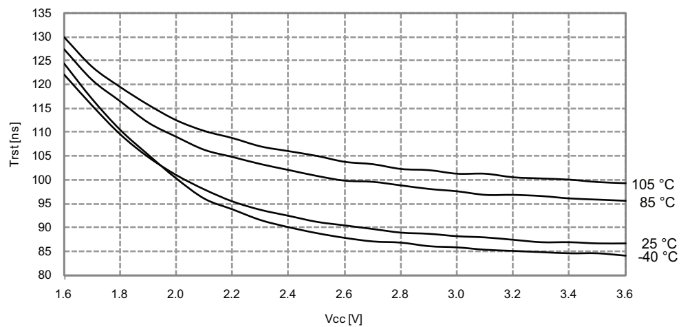
Figure 37-314. Minimum Reset pin pulse width vs. V_{CC}
