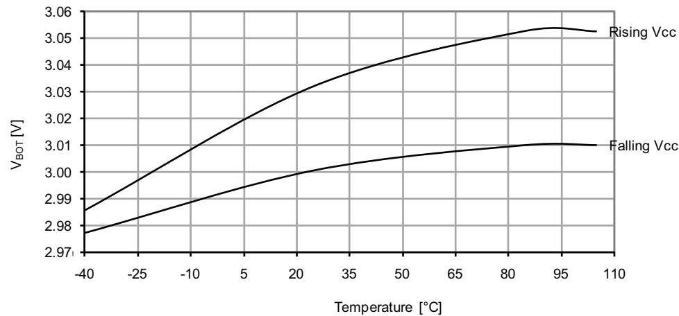
Figure 37-61. BOD thresholds vs. temperature. BOD level = 3.0V.
