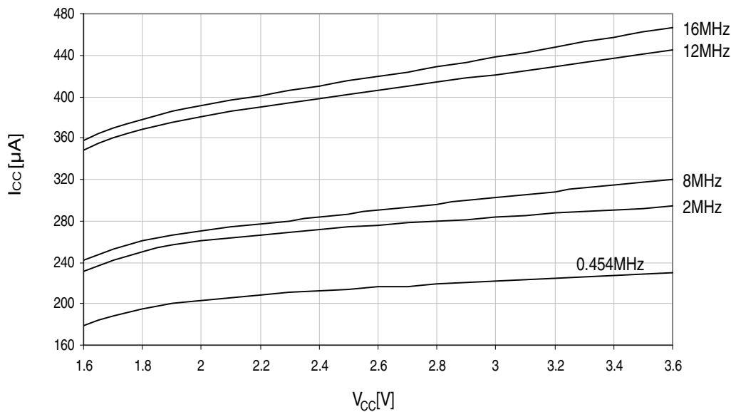
Figure 37-272. Standby supply current vs. V_{CC} . T = 25^{\circ}C , running from different crystal oscillators
