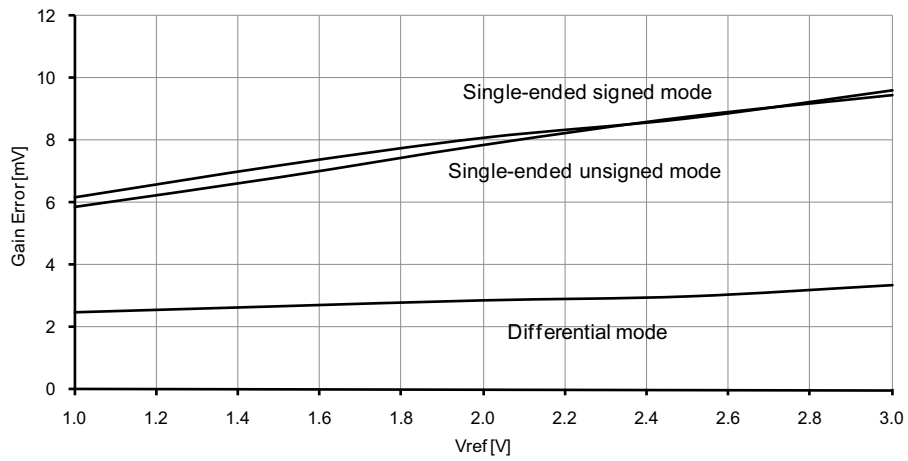
Figure 37-210. Gain error vs. V_{REF} . T = 25^{\circ}\text{C} , V_{CC} = 3.6\text{V} , ADC sampling speed = 500ksps.
