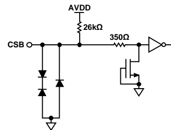
Figure 24. Equivalent CSB Input Circuit
