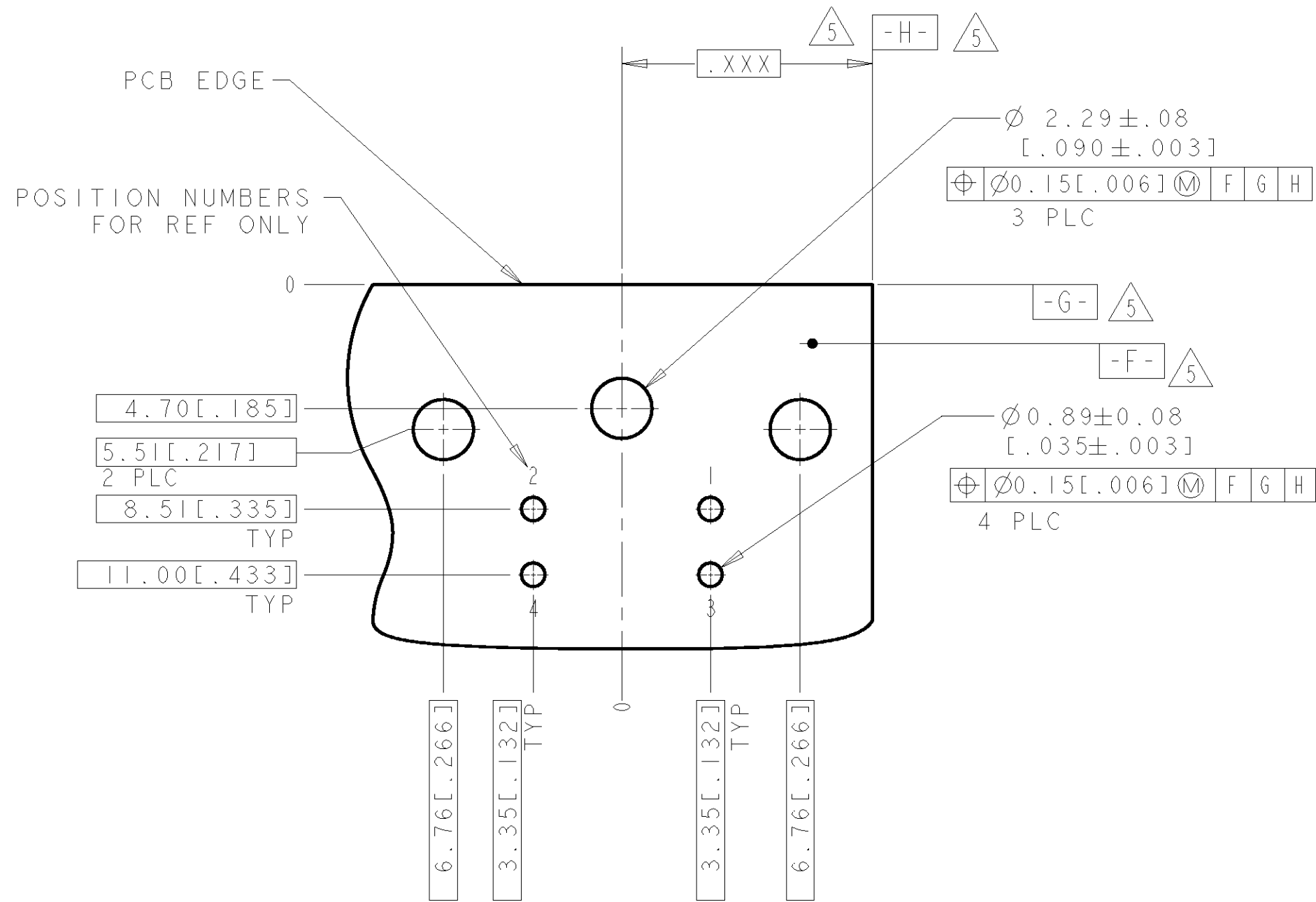
4 PIN PCB LAYOUT BOTTOM VIEW
