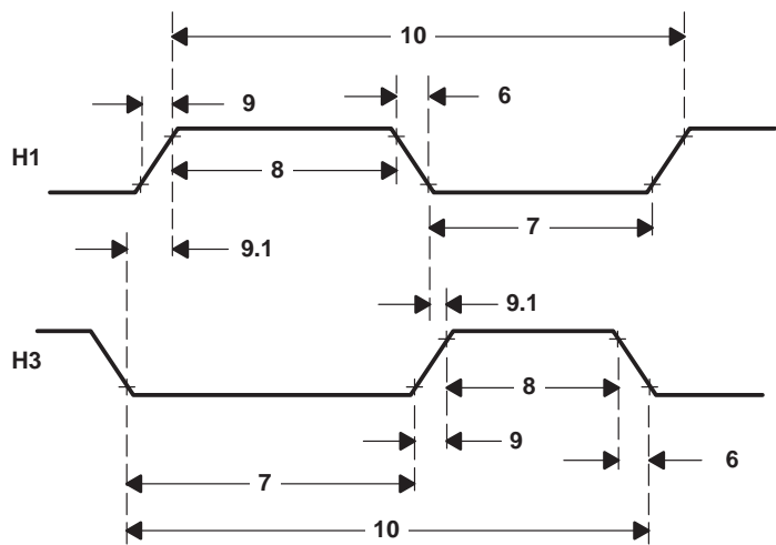
Figure 15. H1/H3 Timing
