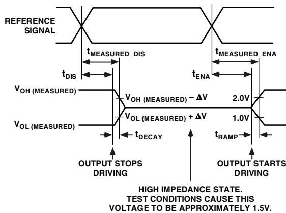
Figure 30. Output Enable/Disable
