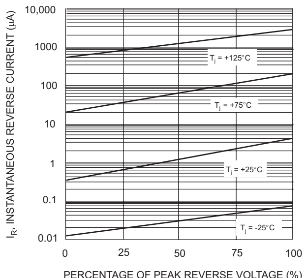
PERCENTAGE OF PEAK REVERSE VOLTAGE (%) Fig. 6 Typical Reverse Characteristics, SB120 thru SB140
