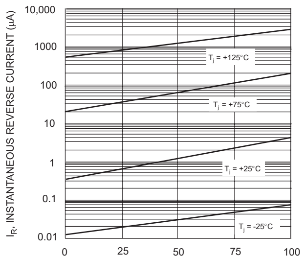
PERCENTAGE OF PEAK REVERSE VOLTAGE (%) Fig. 6 Typical Reverse Characteristics, SB120 thru SB140
