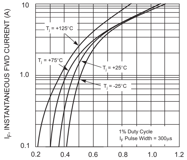
V_F , INSTANTANEOUS FORWARD VOLTAGE (V) Fig. 2 Typical Forward Characteristics - SB120 thru SB140
