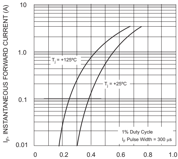
V_F , INSTANTANEOUS FWD VOLTAGE (V) Fig. 3 Typ. Forward Characteristics - SB150 thru SB160
