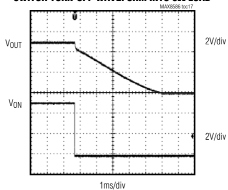
SWITCH TURN-OFF WAVEFORM INTO 5\Omega LOAD
