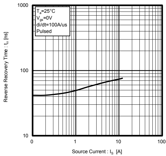
Fig.13 Reverse Recovery Time vs. Source Current
