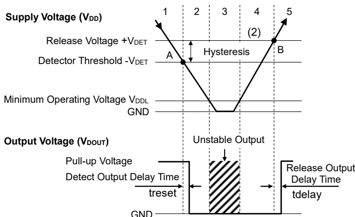
Operation Diagram
