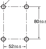
Mounting Holes
