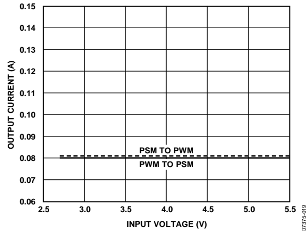
Figure 9. Mode Transition
