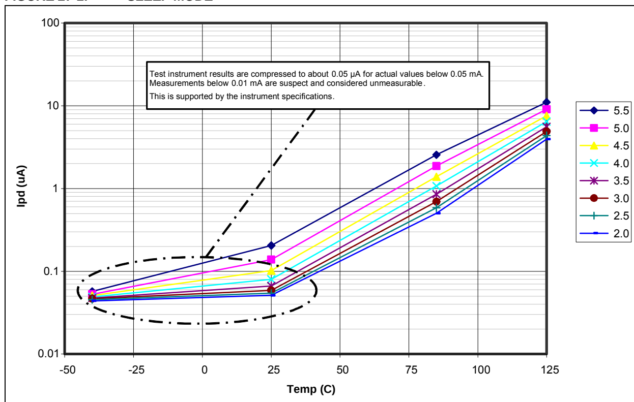
FIGURE 27-1: SLEEP MODE
