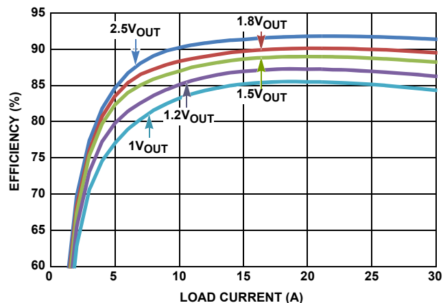
FIGURE 7. EFFICIENCY vs LOAD CURRENT (PARALLEL SINGLE OUTPUT, AS SHOWN IN Figure 19 AT 12V_{\text{IN}} /500kHz)
