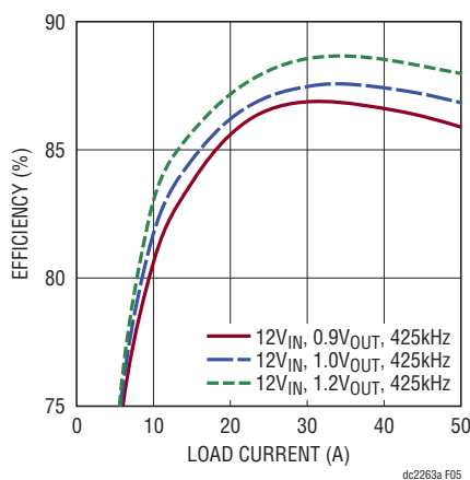
Figure 5. Typical Efficiency Curves DC2263A-B, f_{sw} = 425\text{kHz}
