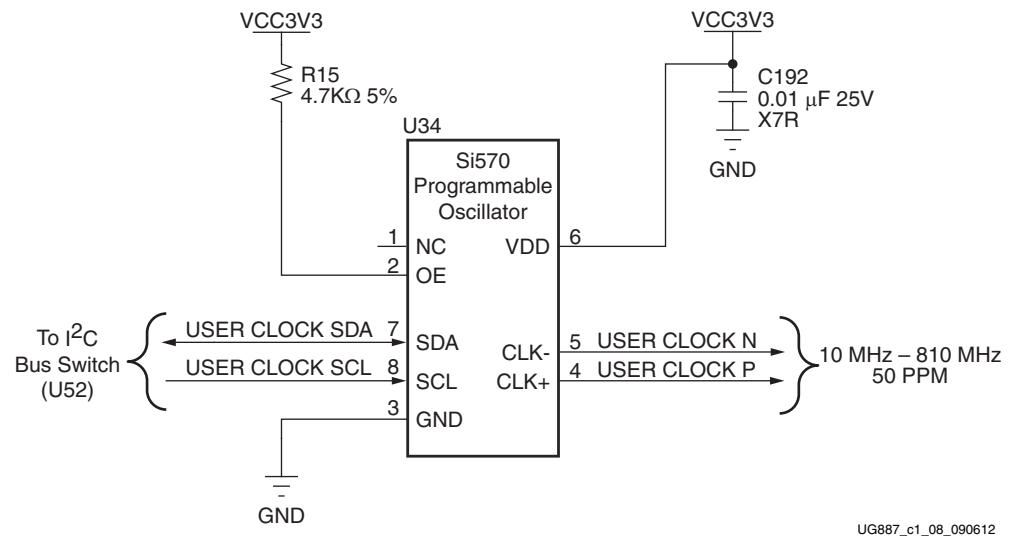
Figure 1-8: User Clock Source
