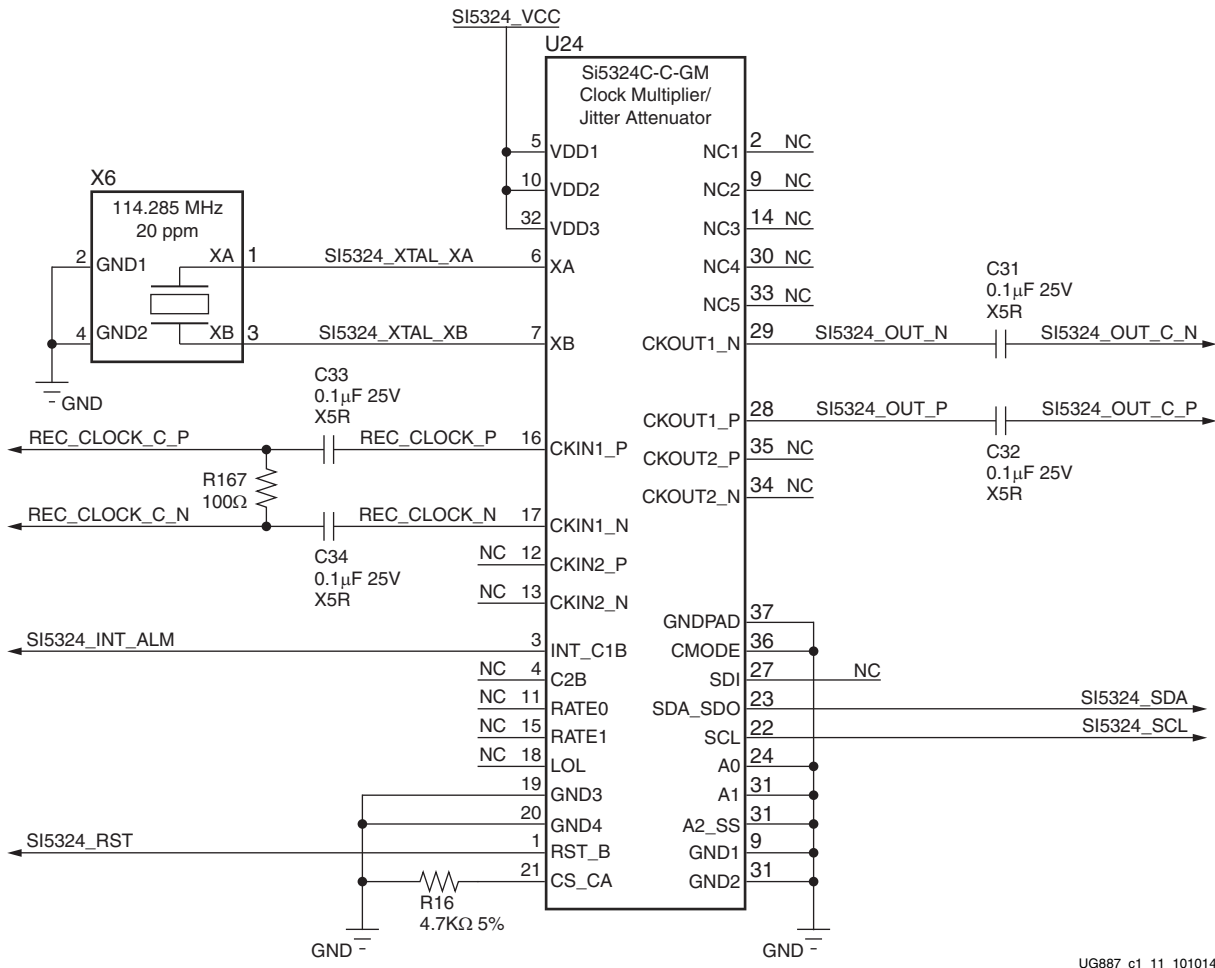
Figure 1-11: Jitter-Attenuated Clock
