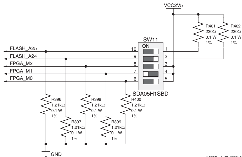
Figure 1-28: Mode Switch
