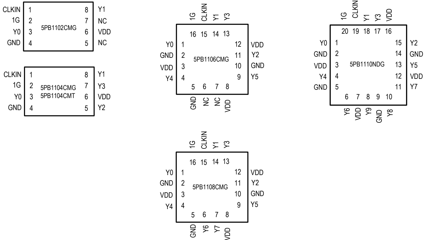
Figure 2. Pin Assignments for DFN/QFPN Packages
