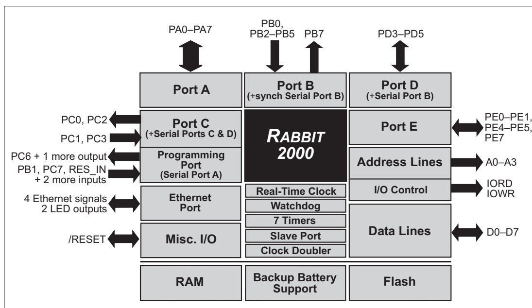
Figure 4. Rabbit Subsystems
