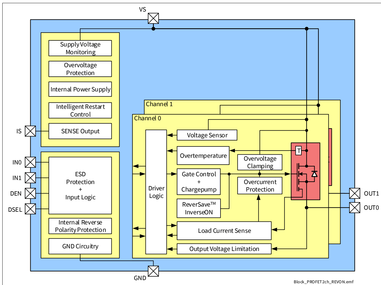
Figure 2 Block Diagram of BTS7010-2EPA
