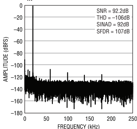
32k Point FFT f_s = 500\text{ksps} , f_{IN} = 20\text{kHz}
