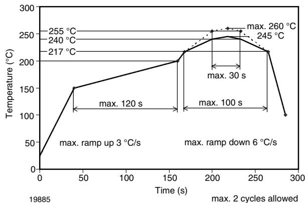
Fig. 16 - Vishay Leadfree Reflow Soldering Profile (acc. to J-STD-020)
