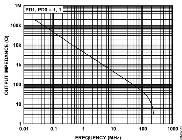
Figure 15. Output Impedance vs. Frequency (Disabled)
