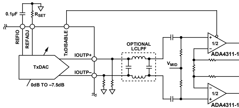
Figure 22. TxDAC Output Directly via Center-Tap Transformer
