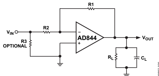
Figure 29. Inverting Amplifier
