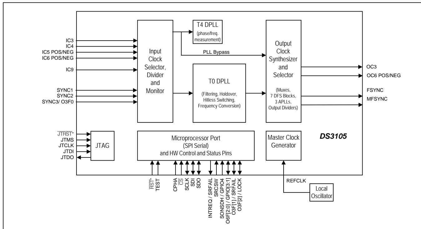
Figure 3-1. Block Diagram
