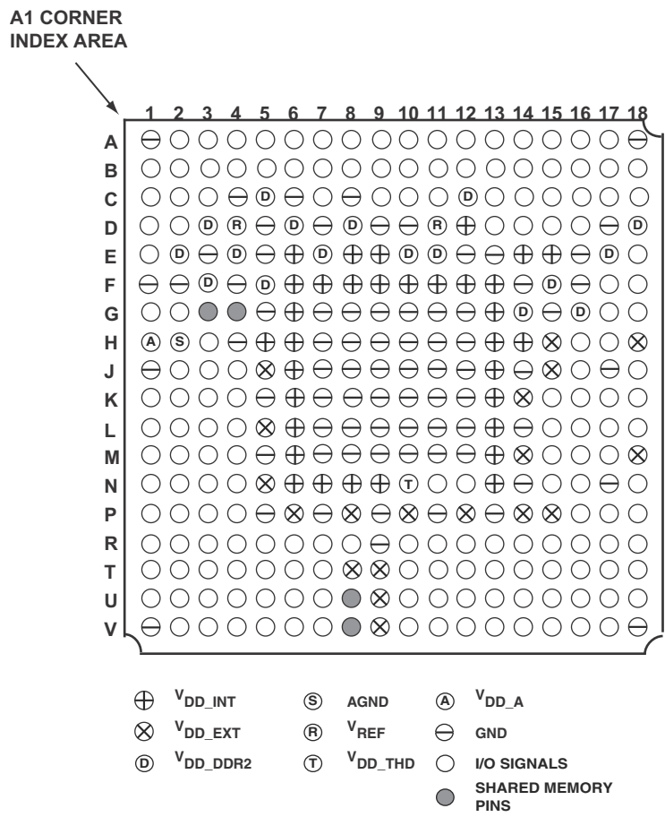
Figure 60. Ball Configuration, Automotive Model
