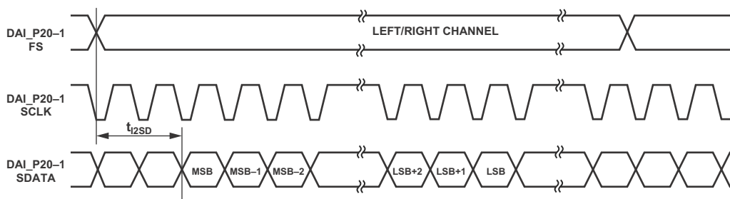
Figure 36. I 2 S-Justified Mode
