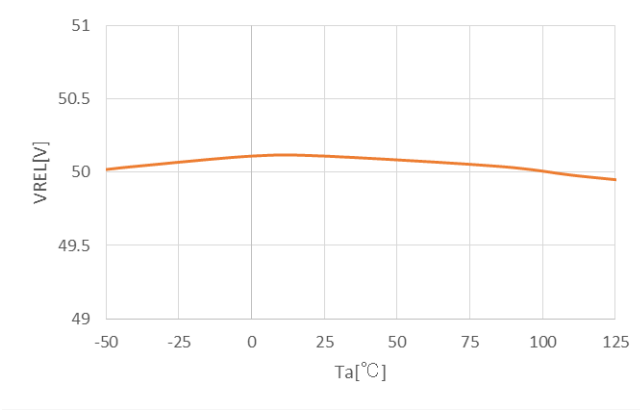
R3160N480A
