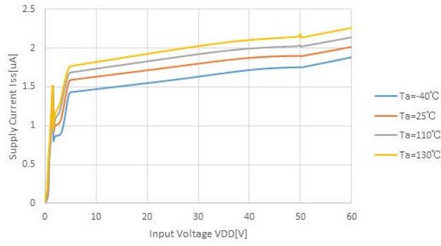
R3160N480A
