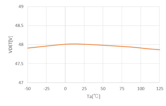
R3160N480A
