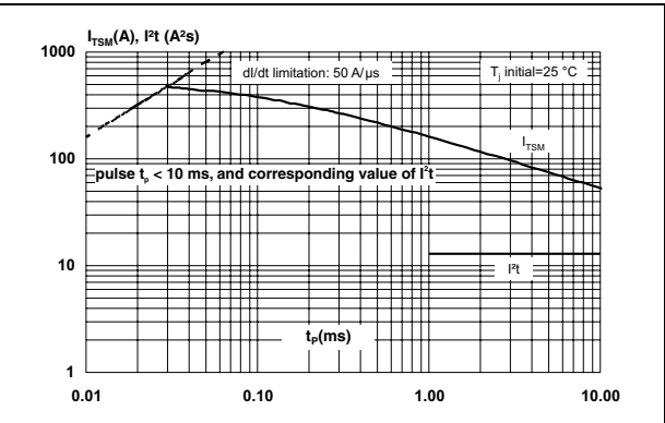
Figure 8. Non-repetitive surge peak on-state current for sinusoidal
