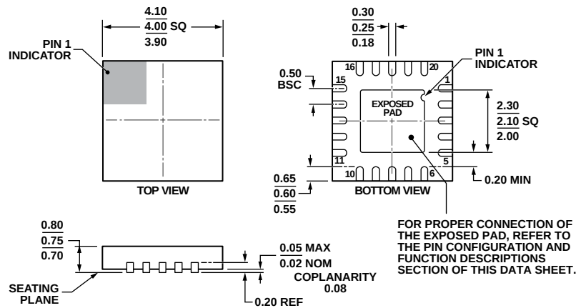
Figure 32. 20-Lead Lead Frame Chip Scale Package [LFCSP_WQ] 4 mm × 4 mm Body, Very Very Thin Quad (CP-20-6) Dimensions shown in millimeters
