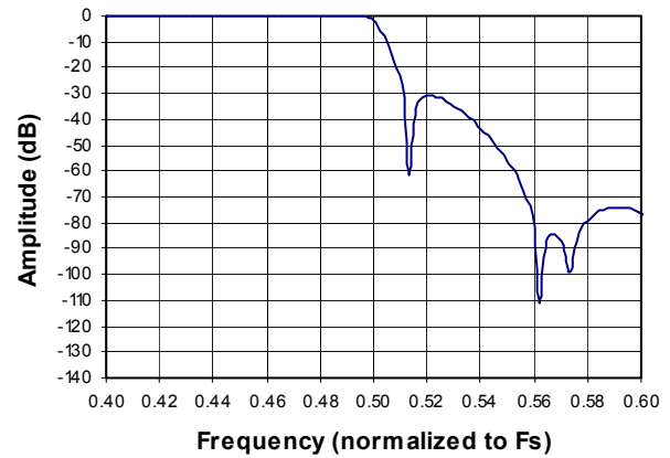
Figure 9. Transition Band
