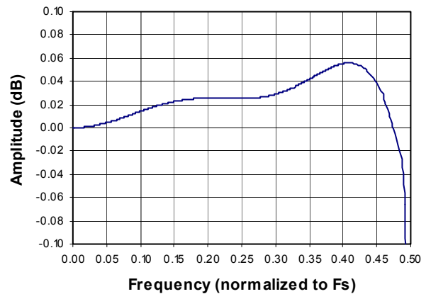
Figure 11. Passband Ripple
