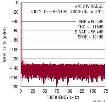
32k Point FFT f_{SAMPL} = 350\text{ksps} , f_{IN} = 2\text{kHz}
