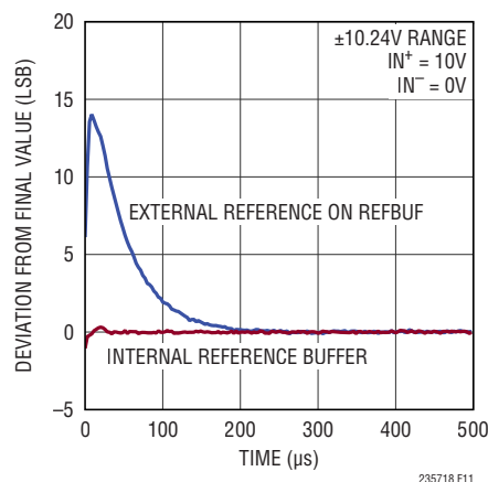
Figure 11. Burst Conversion Response of the LTC2357-18, f_{SMPL} = 350ksps
